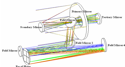
Figure 5 Optics design
