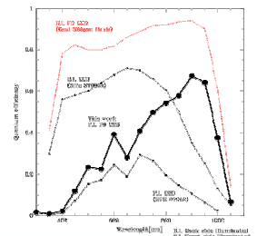
Figure 6 Quantum Efficiency
